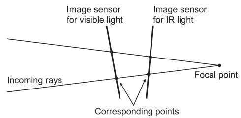
Fig. 10 The virtual optical path are common for all image sensors. Due to the misalignments, an incoming ray is projected on the different pixel of the image sensors.
